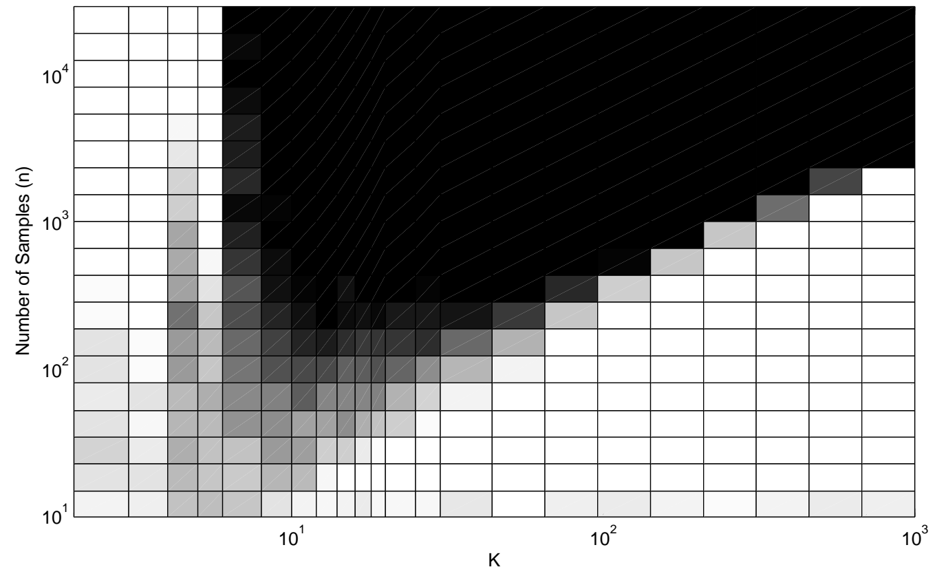
S4 – Averaging
