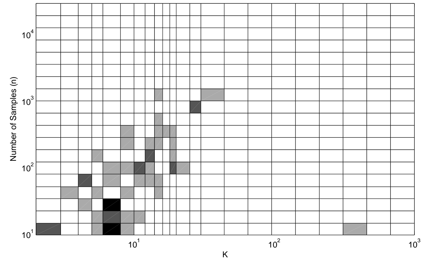
S8 – Voting
