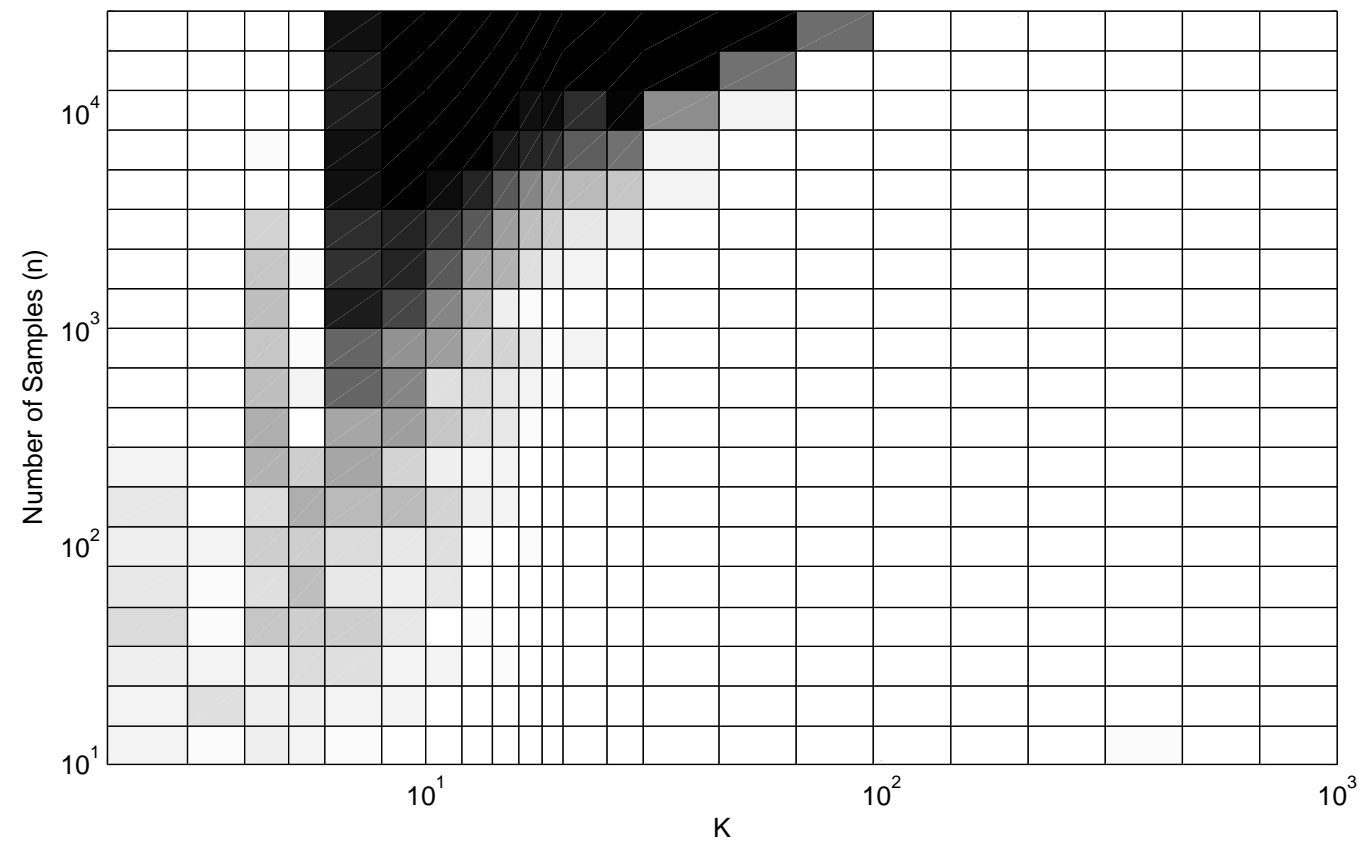
S8 – Averaging
