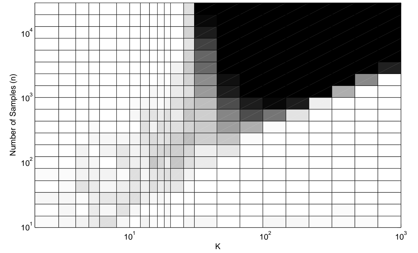
S4 – Voting
